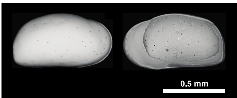
Images 2a & b: Calcitic shells of deep-sea ostracod genus Krithe . Shells of this genus were used for geochemical analysis. Note that these are just for illustration purpose and not the specimens from the studied area. Photo credit: Moriaki Yasuhara
