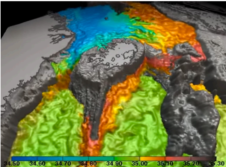
Image 1: Atlantic meridional overturning circulation. Image credit: NASA/Goddard Space Flight Center Scientific Visualization Studio ( http://svs.gsfc.nasa.gov/3884 )
