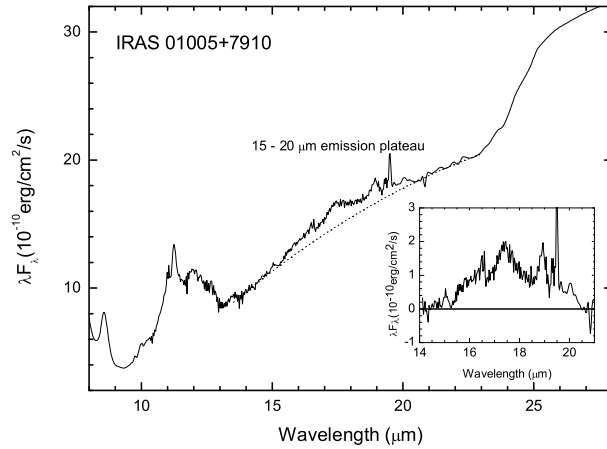
Figure 8. Spitzer IRS spectrum of the PPN IRAS 01105+7910 showing the 17 \mu\text{m} plateau emission. Figure adapted from Zhang & Kwok (2010).
