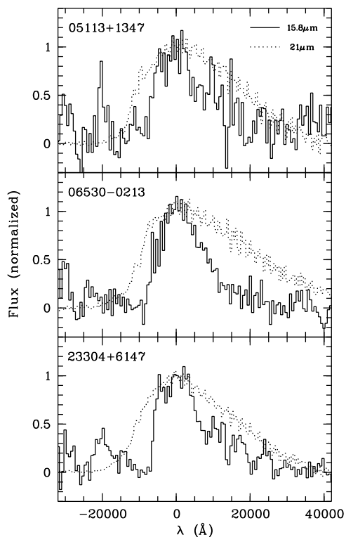
Figure 5. Comparison of the profiles of the 21 and 15.8 \mu\text{m} features in 3 PPNs. Figure adapted from Zhang & Kwok (2010).
